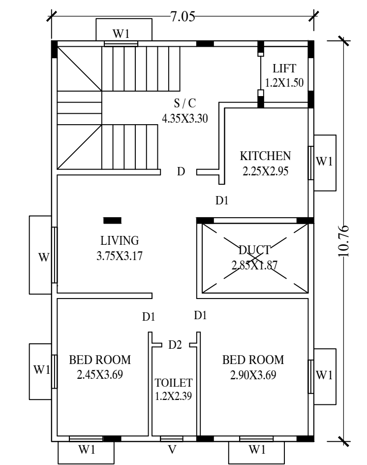
PROPOSED TYPICAL GROUND, FIRST & SECOND FLOOR PLAN
